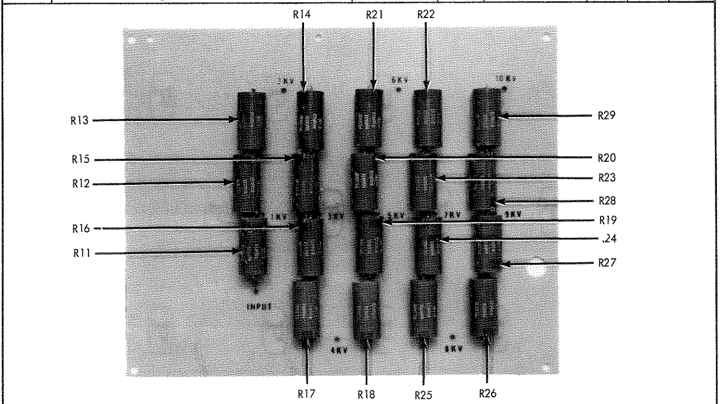
Figure 5-3. DIVIDER ASSEMBLY
